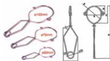
LX06 Pipeform Anchor Stainless Steel Wire Size: 2" / 3" / 4" MBL: 27kn
